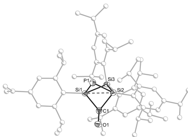
Figure 1. Molecular structure of the anionic moiety in [\text{K}(2,2,2\text{-crypt})]\textbf{1}\cdot 2\text{C}_6\text{H}_6 (ellipsoids set at 50 % probability; hydrogen atoms, crystal solvent, and second component of positional disorder of phosphide vertex and carbonyl (1:1) omitted for clarity). Atoms of Tip groups shown as spheres of arbitrary radius. Selected interatomic distances [Å] and angles [°]: P1–Si1 2.215(4) , P1–Si2 2.174(4) , Si1...Si2 2.618(1) , Si1–Si3 2.375(1) , Si2–Si3 2.375(1) , Si1–C1 2.009(15) , Si2–C1 2.005(16) , C1–O1 1.204(15) ; Si1–P1–Si2 73.22(11) , Si1–C1–Si2 81.4(6) , P1–Si1–Si3 94.16(9) , P1–Si1–C1 82.7(4) , P1–Si2–Si3 95.20(9) , P1–Si2–C1 83.9(4) , Si1–Si3–Si2 66.89(2) .
