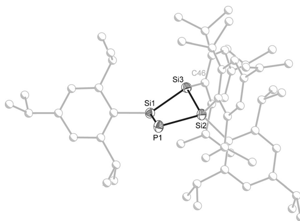
Figure 2. Molecular structure of the anionic moiety in [K(18\text{-crown-6})]2 \cdot 0.5 C_7H_8 (ellipsoids set at 50% probability; hydrogen atoms are omitted for clarity; atoms of Tip groups are pictured as spheres of arbitrary radius. Selected interatomic distances [Å] and angles [ ^\circ ]: P1-Si1 2.156(1) , P1-Si2 2.263(1) , Si1-Si3 2.212(1) , Si2-Si3 2.364(1) ; Si1-P1-Si2 80.785(16) , P1-Si1-Si3 101.669(18) , P1-Si2-Si3 94.108(16) , Si1-Si3-Si2 77.427(15) , Si1-Si3-C46 128.46(4) , Si1-Si3-C46 126.75(4) .
